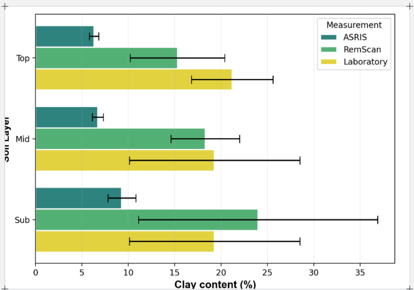
Figure 3: Qualitative comparison of predicted clay content from ASRIS, RemScan and an accredited laboratory across three sublayers for a test farm. Error bars indicate the standard deviation. ASRIS estimates were averaged from 90 m gridded data.
