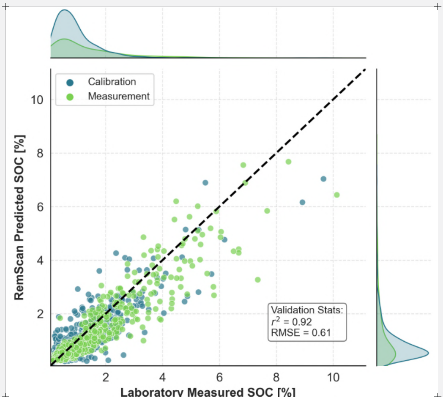
Figure 2: Predictive performance of the model built using GXLab's Australian SOC library. The black dotted line indicates the y=x line. The calibration dataset consists of the best-matching samples taken from GXLab's mid-IR library, while the validation samples include those taken as part of this study.
